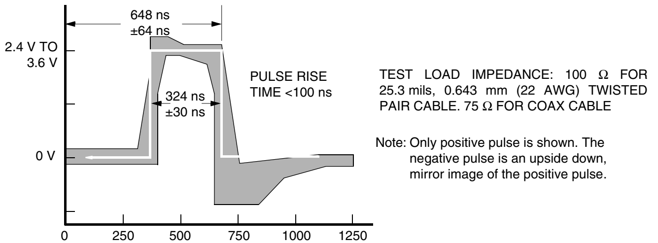
Figure 26. TOTA/C Card Output Waveform
