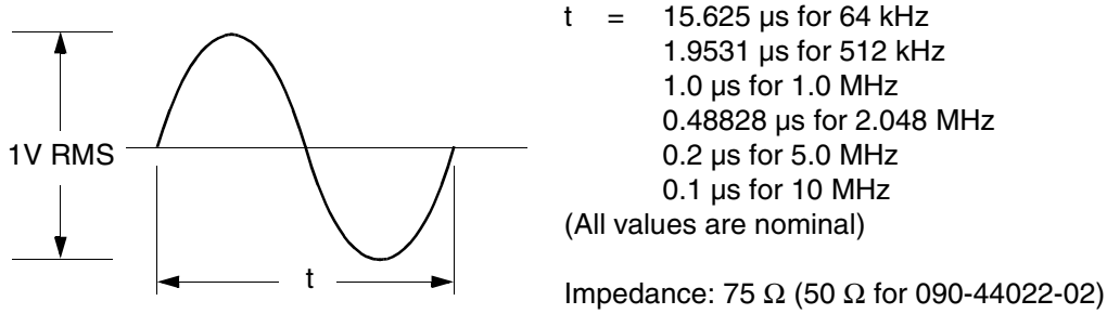
Figure 20. TOAA/C Card Output Waveform
